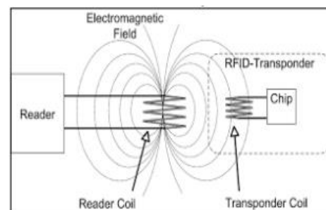
Fig. 2: Basic Functioning of Radio Frequency Identification (RFID)
