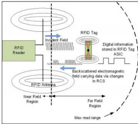
Fig. 3: Radio Frequency Identification (RFID) Communication
